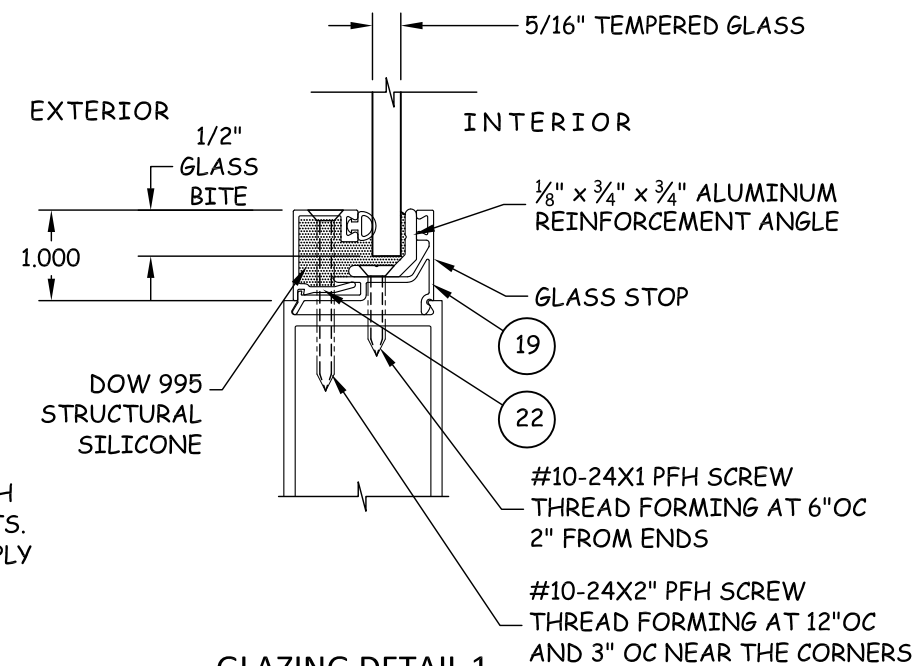
GLAZING DETAIL 1
